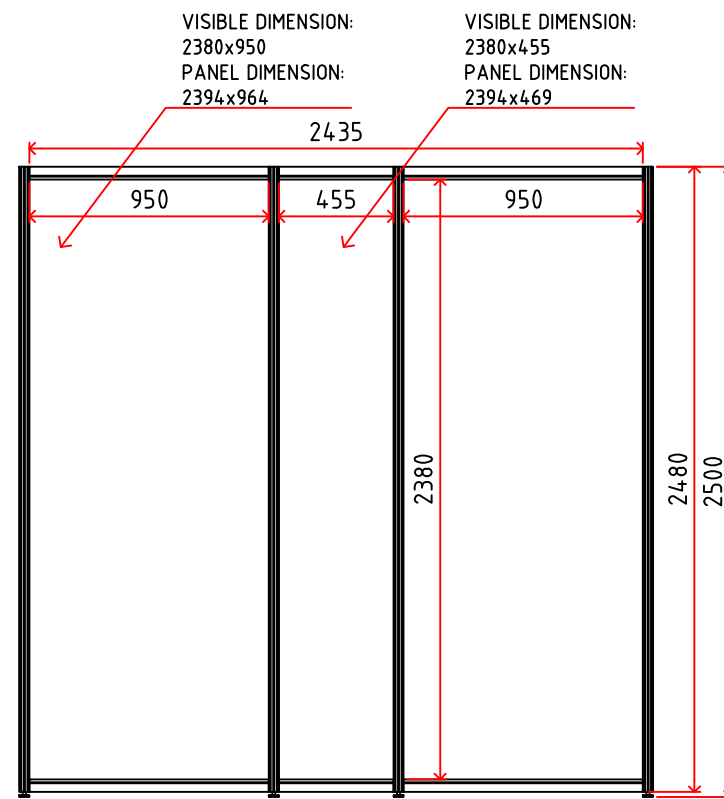
BACK WALL
