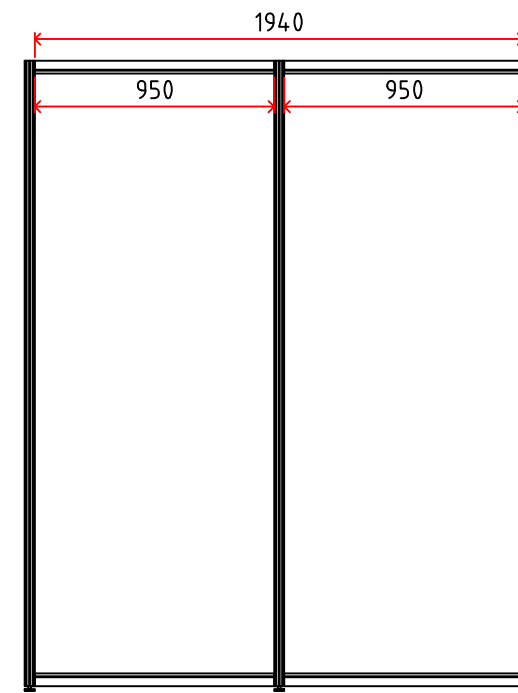
RIGHT WALL
