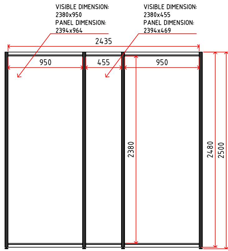
BACK WALL
